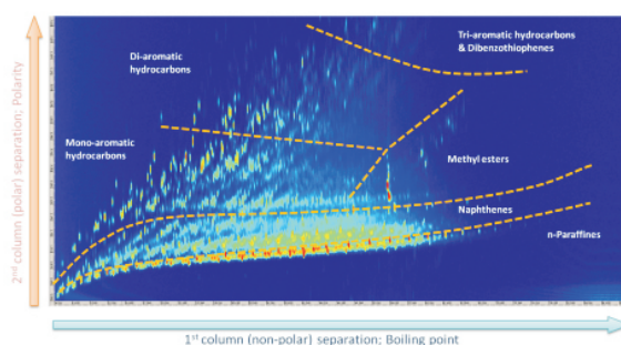
50Hz Acquisition Rate Capability for GCxGC
